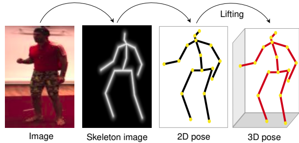
Figure 1. 3D pose estimation pipeline. Our approach jointly learns to estimate 3D pose from an image via intermediate representations of 2D pose. The pipeline is embedded within a larger network for end-to-end training.
