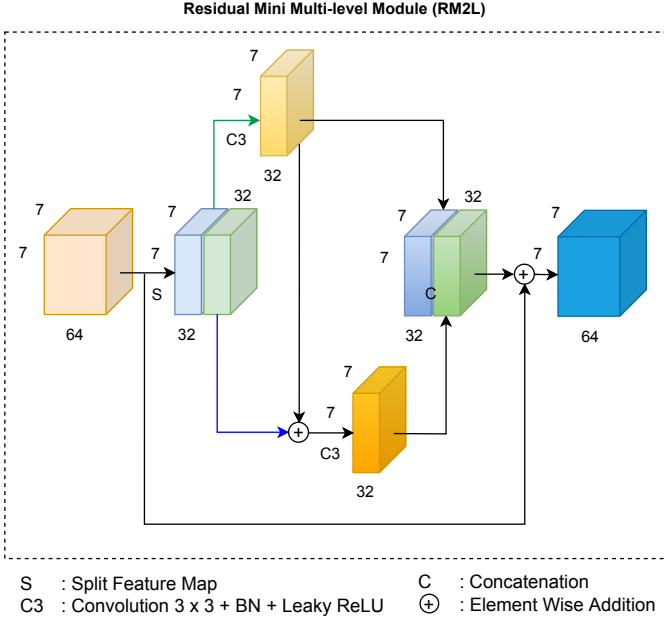
Fig. 2. The proposed Residual Mini Multi-level module.
