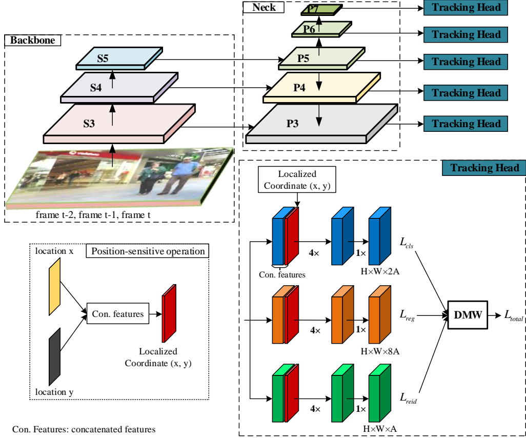
Fig. 2. The overall architecture consists of three parts: backbone network, neck, and tracking head. The backbone network served as feature extraction takes the current frame and past frame as input. The neck part forming a pyramid feature \{P3, P4, P5, P6, P7\} takes three feature maps \{S3, S4, S5\} from stage 3, stage 4, and stage 5 of the backbone network to gather low-level and high-level feature. Each tracking head includes three branches: classification branch, regression branch, and re-ID branch. 4\times denotes four convolutional layers in which each layer contains one 3\times 3 convolution operation following by Group Normalization and ReLU activation function. 1\times denotes one convolution operation without normalization and activation function. H, W is the height and width of the feature map. A indicates the number of anchor boxes per location. L_{cls}, L_{reg}, L_{reid}, L_{total} are classification, regression, re-ID loss, and total loss, respectively. DMW is the dynamic multi-loss weighting function.
