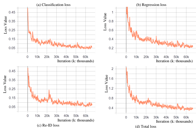
Fig. 1. The learning paces of regression, classification, and re-ID tasks with the proposed network (Fig. 2 without using the proposed DMW) are shown. The model is trained with hard weighting factors.
