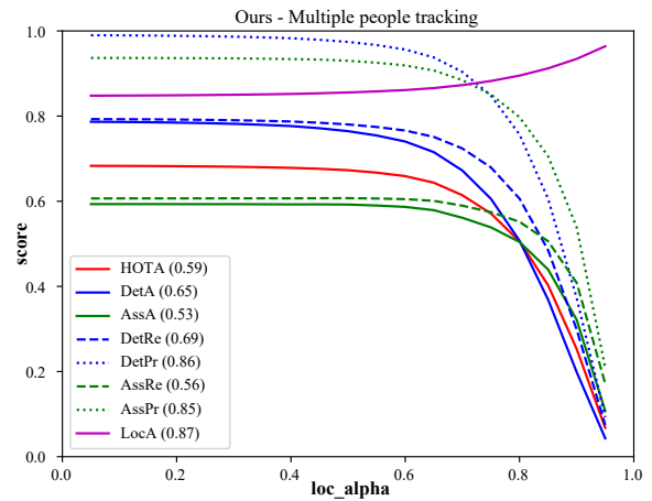
Fig. 3. HOTA score and error components at different threshold loc_alpha.
