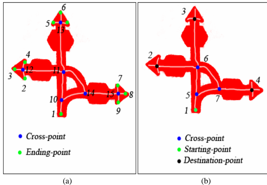
Figure 10: Key points of arrow region
