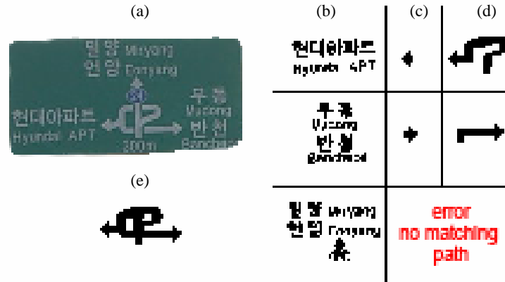
Figure 15: Failed recognition example. Output consists of extracted candidate (a), direction label (b), arrowheads(c), and extracted paths (d)
