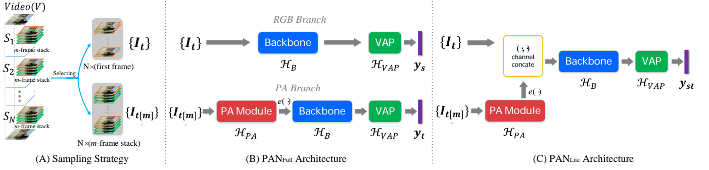
Fig. 3. The overall architecture of Persistent Appearance Network (PAN). It has two network variants: (B) PAN_{Full} - “divide and conquer”, i.e. , capturing the spatial and temporal semantics separately; (C) PAN_{Lite} - “unified and efficient”, i.e. , extracting the spatial and temporal semantics simultaneously.
