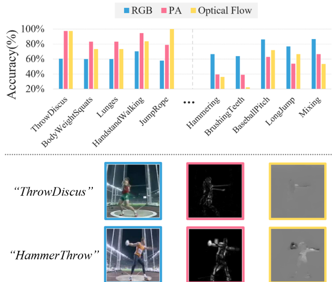
Fig. 5. Top part: The top 5 action classes that show the greatest difference in terms of accuracy between the input modality RGB and PA, and the performance of optical flow in these classes is also plotted for comparison. Bottom part: Input modality visualization of the two classes that are most easily misclassified by RGB. Best viewed in color and zoomed in.
