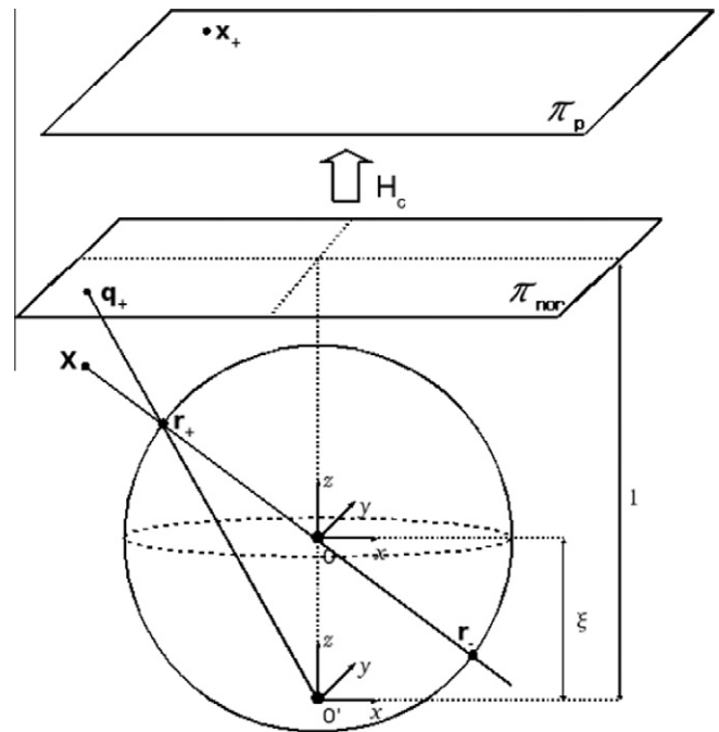
Fig. 1. Projection of a 3D point in the image plane using the sphere camera model.
