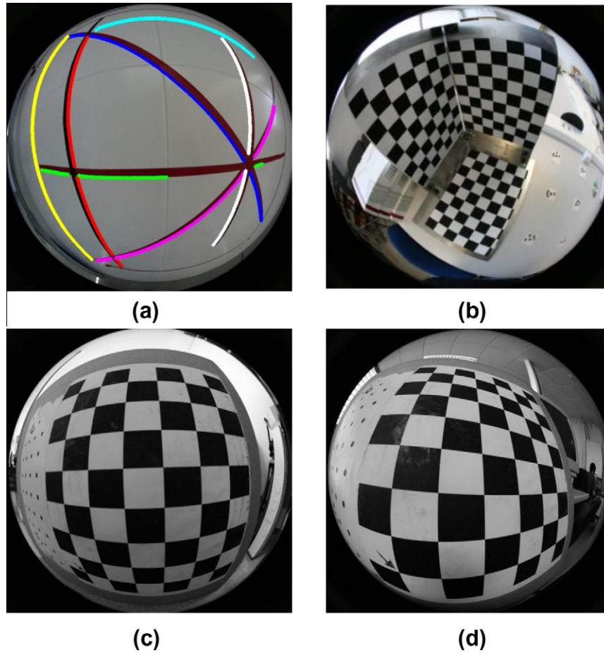
Fig. 10. Some images used to calibrate the fish-eye system. (a) Sphere-lines. (b) DLT-like approach. (c and d) Sphere-2DPattern and Distortion-2DPattern approaches.
