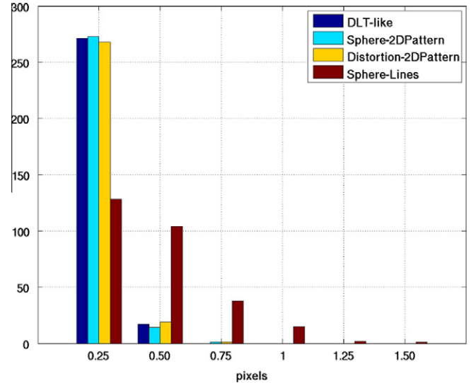
Fig. 9. Number of reprojected points within an error distance in pixels using a hyper-catadioptric system.
