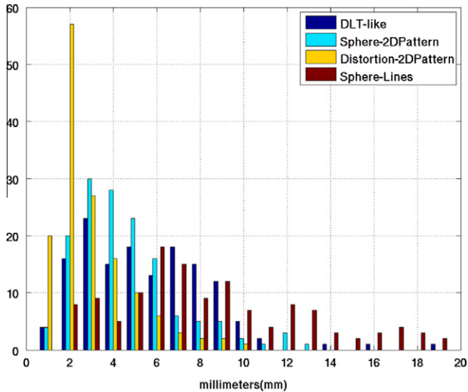
Fig. 16. Number of reconstructed 3D points within an error distance in millimeters using an unknown-shape system.
