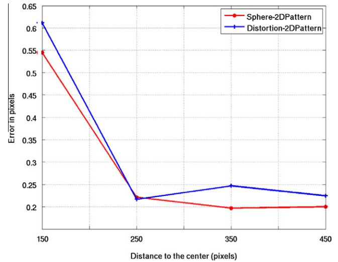
Fig. 24. Reprojection error in pixels. The horizontal axis represents the different radii r .
