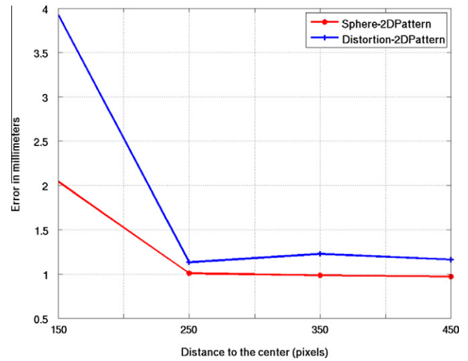
Fig. 23. 3D reconstruction error in millimeters. The horizontal axis represents the different radii r .
