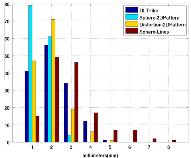
Fig. 20. Number of reconstructed 3D points within an error distance in millimeters using a non-central hyper-catadioptric system.
