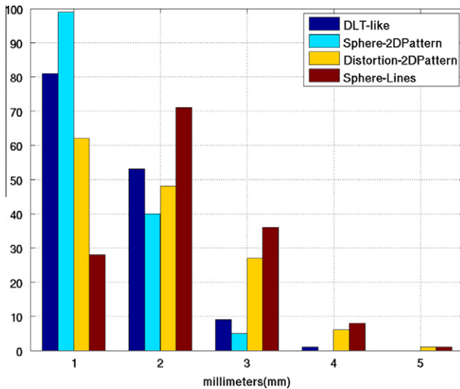
Fig. 8. Number of reconstructed 3D points within an error distance in millimeters using a hyper-catadioptric system.
