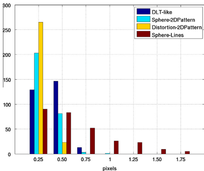
Fig. 17. Number of reprojected points within an error distance in pixels using an unknown-shape system.
