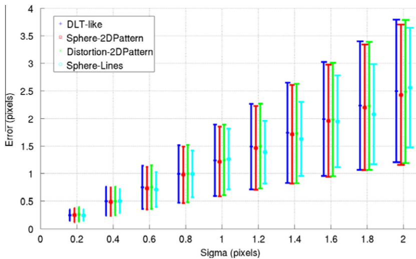
Fig. 4. Reprojection error in pixels as a function of noise ( \sigma ) corresponding to the paracatadioptric system.
