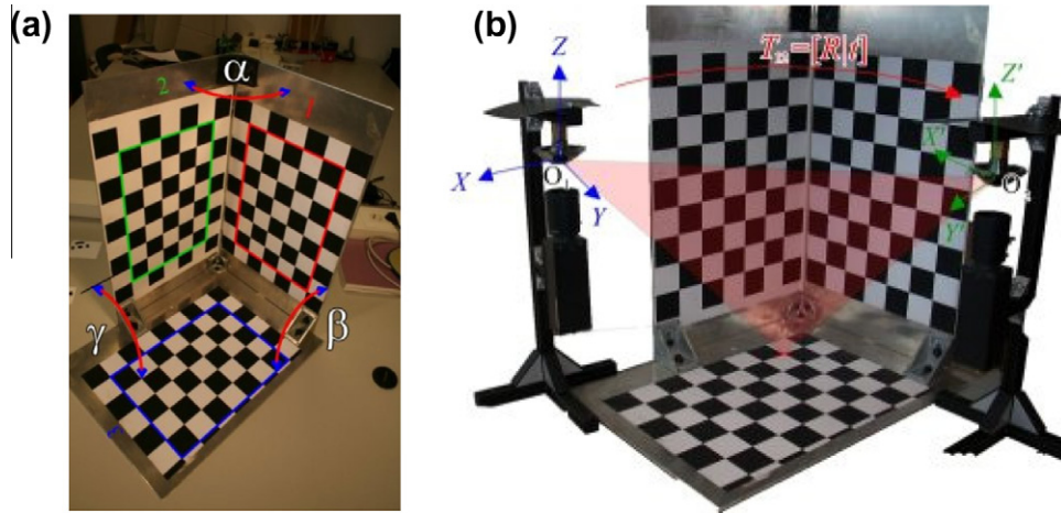
Fig. 5. (a) 3D pattern. (b) SfM configuration to test the calibrations.
