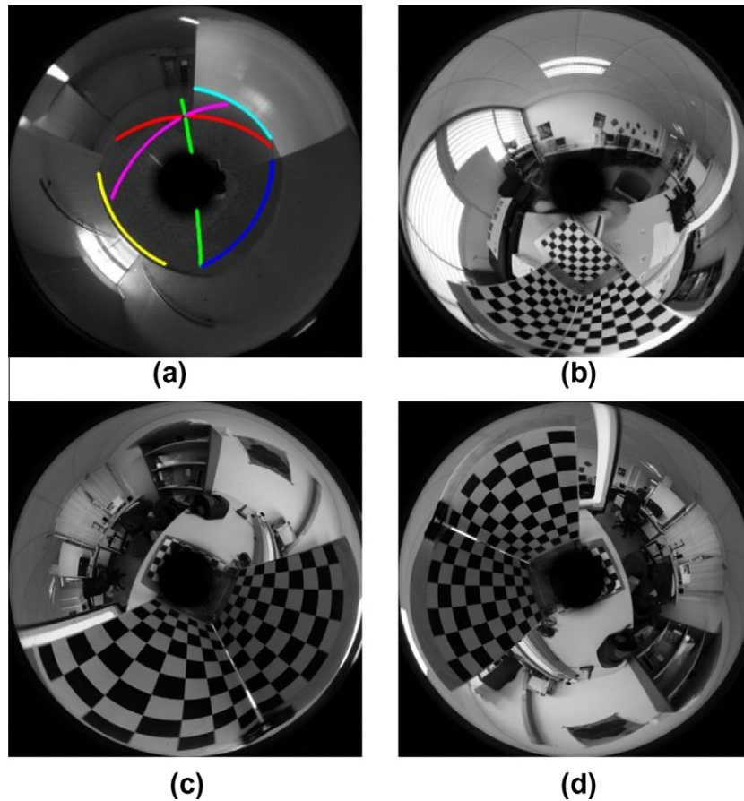
Fig. 14. Some images used to calibrate the unknown-shape catadioptric system. (a) Sphere-Lines. (b) DLT-like approach. (c and d) Sphere-2DPattern and distortion-2DPattern approaches.
