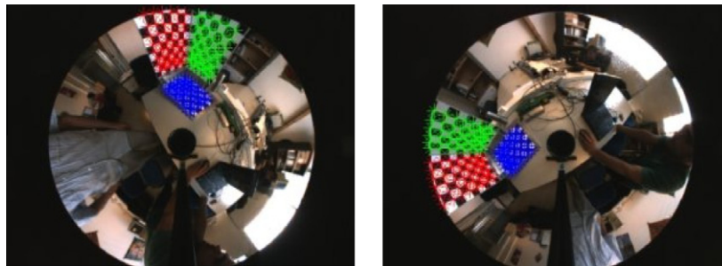
Fig. 19. Images used in the SfM experiment with reprojected points superimposed (non-central hyper-catadioptric).
