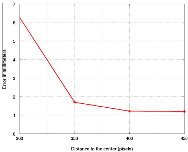
Fig. 26. 3D reconstruction error in millimeters. The horizontal axis represents the different radii r .
