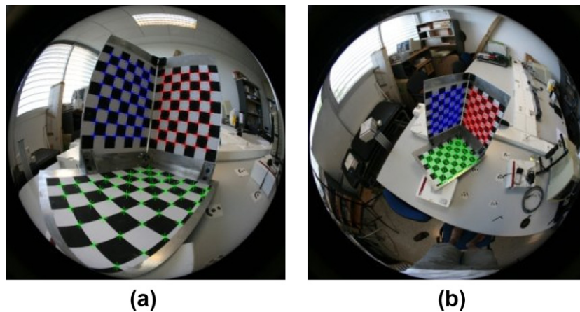
Fig. 11. Images used in the SfM experiment with reprojected points superimposed (fish-eye).
