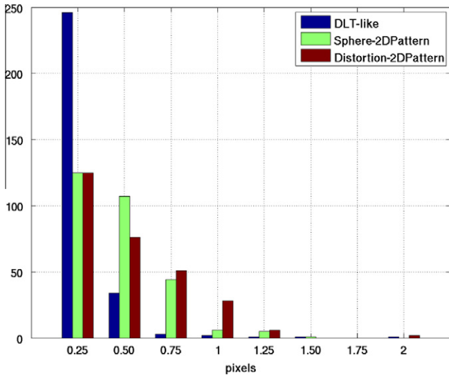
Fig. 13. Number of reprojected points within an error distance in pixels using a fish-eye lens.
