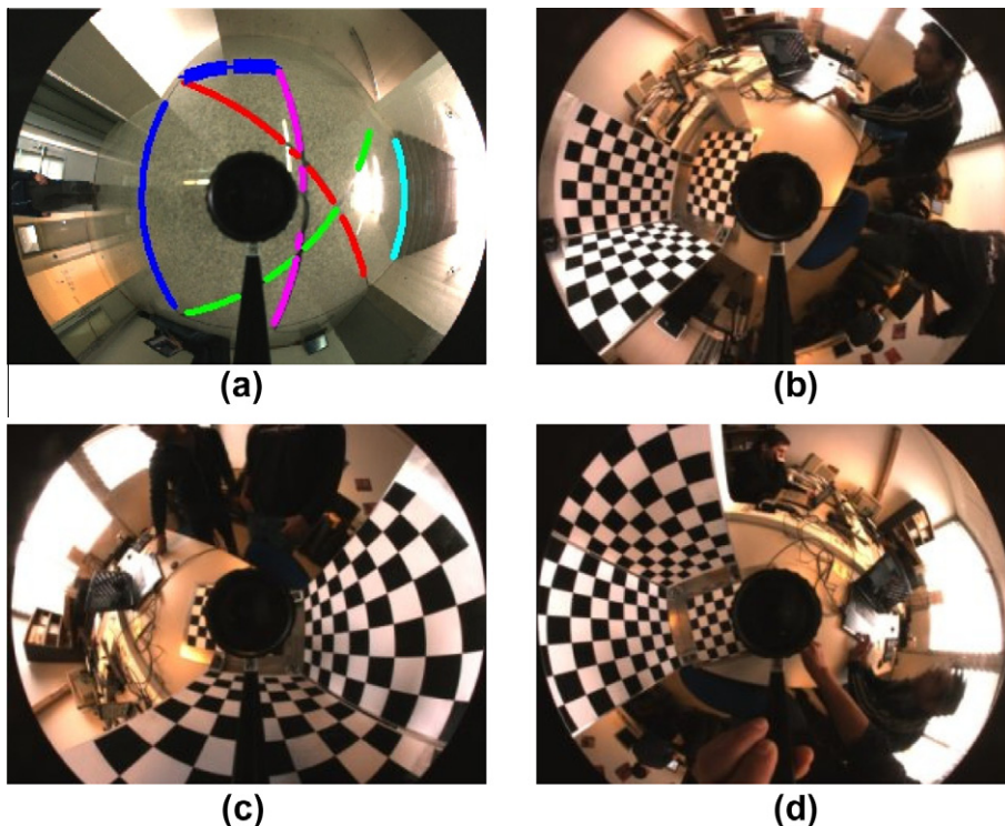
Fig. 6. Some images used to calibrate the hyper-catadioptric system. (a) Sphere-Lines. (b) DLT-like approach. (c and d) Sphere-2DPattern and Distortion-2DPattern approaches.
