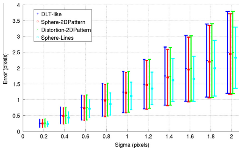
Fig. 3. Reprojection error in pixels as a function of noise ( \sigma ) corresponding to the hypercatadioptric system.
