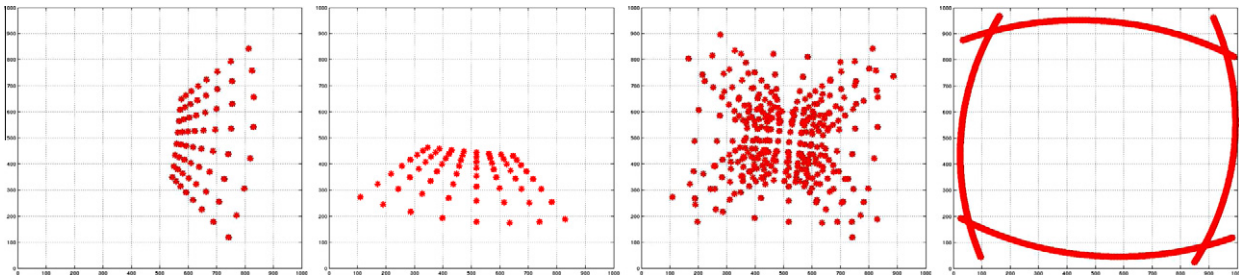
Fig. 2. Synthetical images used by the calibration methods. Sphere-2DPattern and Distortion-2DPattern approaches use five images similar to (a) and (b). (c) DLT-like approach uses a single image containing 5 planar patterns. (d) Sphere-lines approach use 4 image lines.
