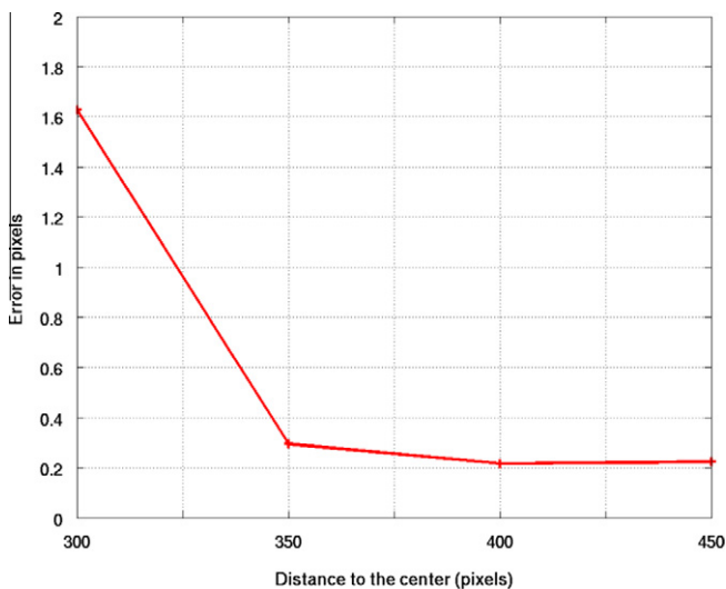
Fig. 27. Reprojection error in pixels. The horizontal axis represents the different radii r .
