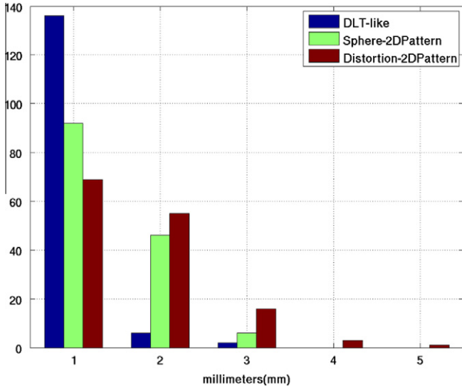
Fig. 12. Number of reconstructed 3D points within an error distance in millimeters using a fish-eye lens.
