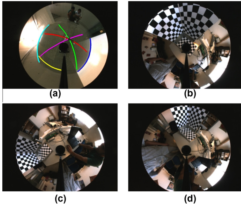
Fig. 18. Some images used to calibrate the non-central catadioptric system. (a) Sphere-Lines. (b) DLT-like approach. (c and d) Sphere-2DPattern and Distortion-2DPattern approaches.
