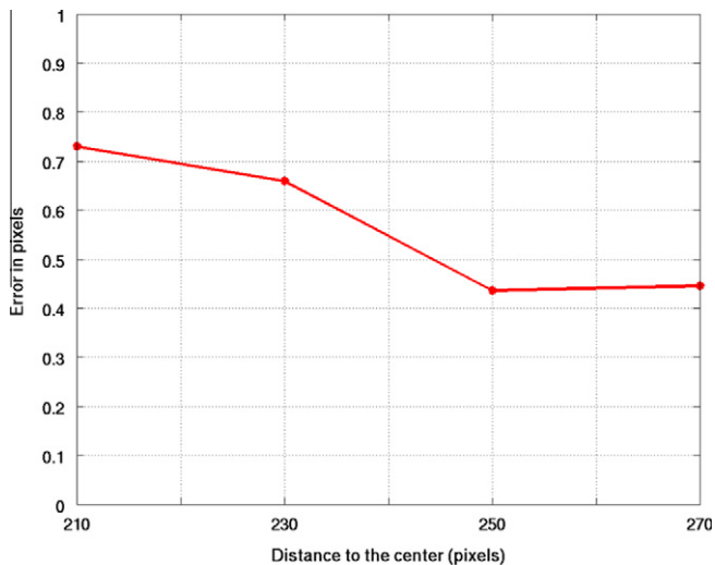
Fig. 30. Reprojection error in pixels. The horizontal axis represents the different radii r .
